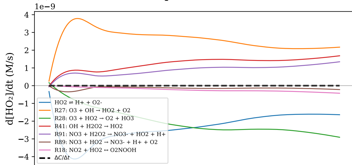
(a) HO 2 [final=148.00 pM]
