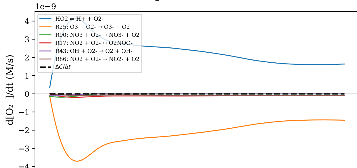
(c) O 2 - [final=30.82 pM]
