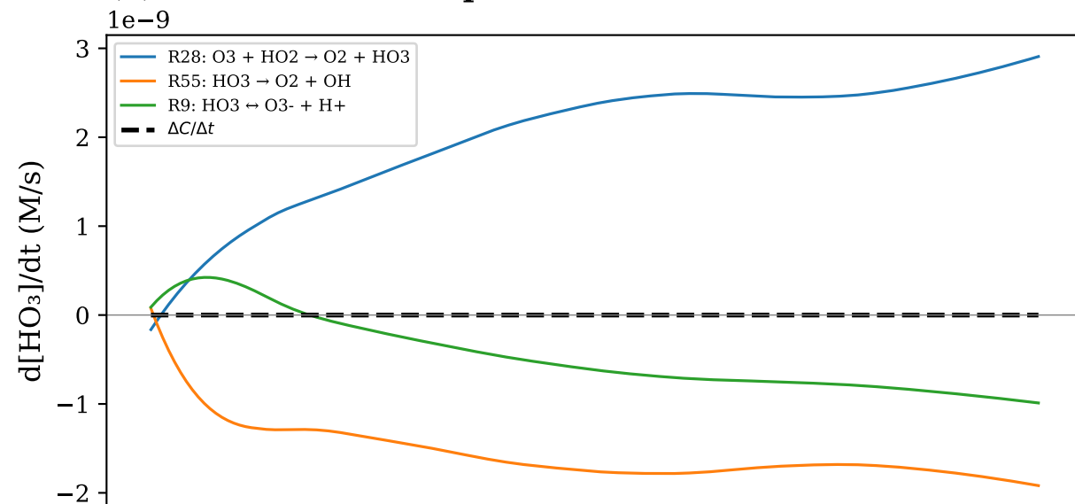
(b) HO 3 [final=0.02 pM]
