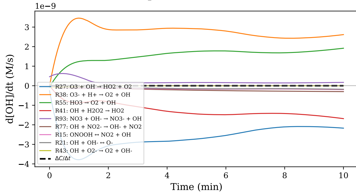
(e) OH [final=0.91 pM]
